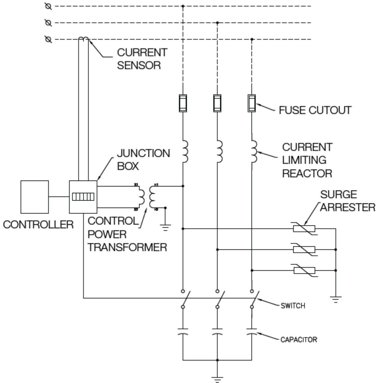
FIGURE 1A: POLE MOUNTED AUTO SWITCHED CAPACITOR BANKS CIRCUIT DIAGRAM
